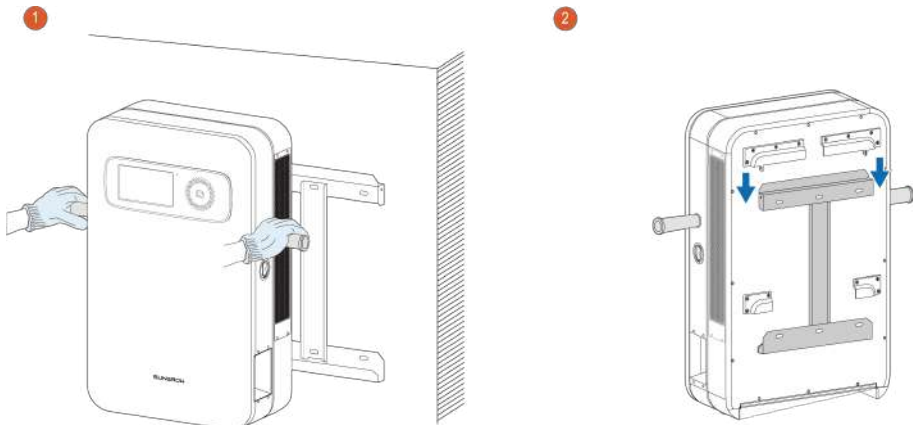
figure 2-10 Charger installation
