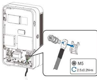
figure 2-17 Connect the cable connection terminal
