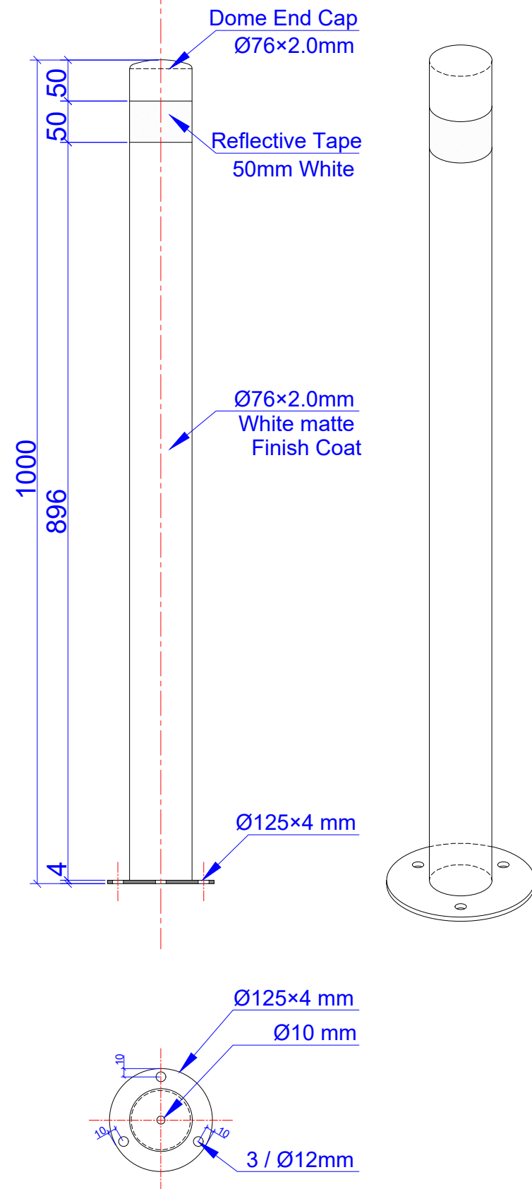
BOLW76 76mm x 1000mm Surface Mounted Stainless Steel White Bollard with Fixing Kit
