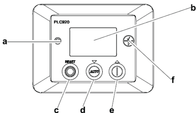
Control module
