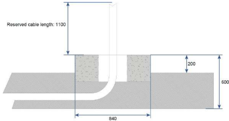
Figure 3-1 Section View of the Foundation(mm)
