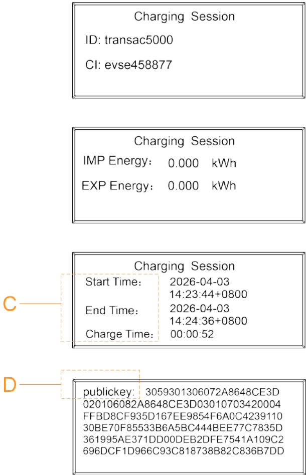
Figure 7-6 Charging End
