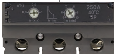
Adjustable-thermal, Adjustable-magnetic
