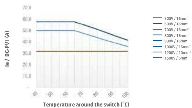
Switch SI32 4H DC-PV1 Open Type
