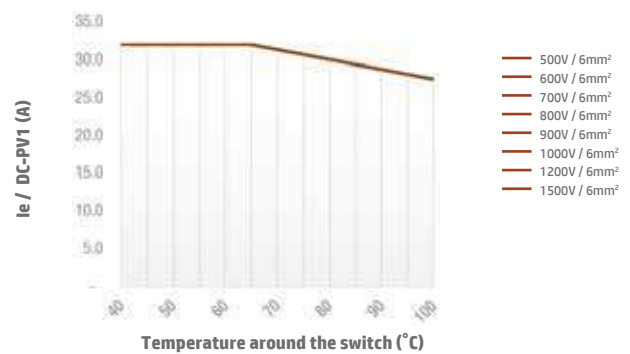
Switch SI32 4B/4S/4T DC-PV1 Open Type
