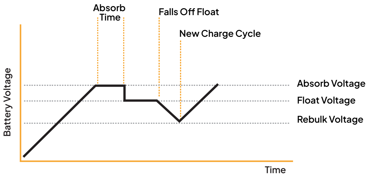
Figure 6: Battery Charge Profile Illustrated
