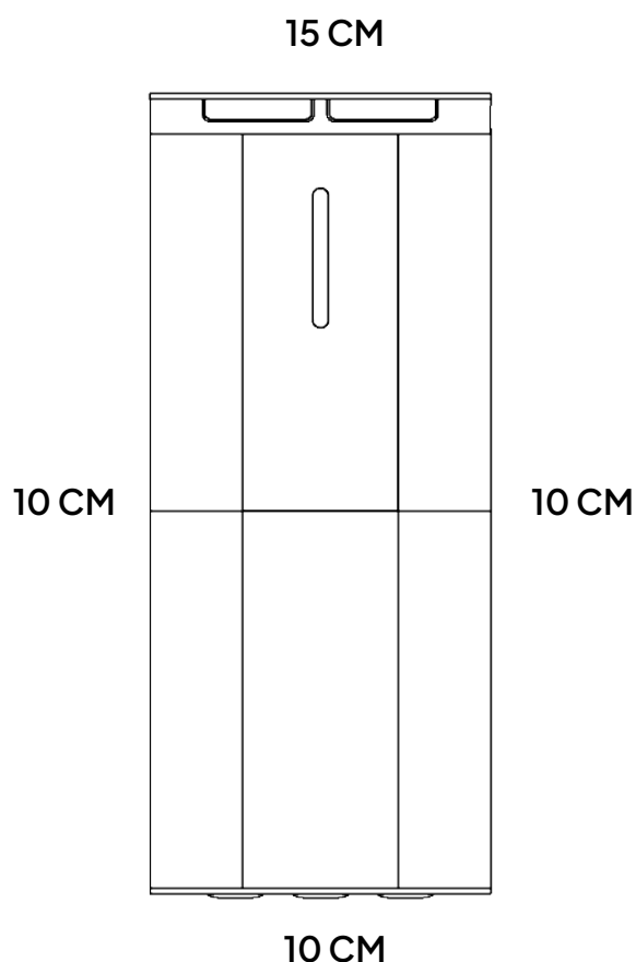
Figure 1B: SRX Mounting Clearances
