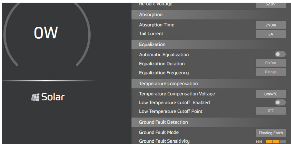
Figure 11: Earth Fault Sensitivity Adjustment
