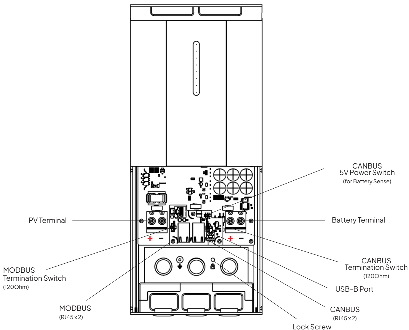
Figure 2: SRX Access Panel Screw Locations
