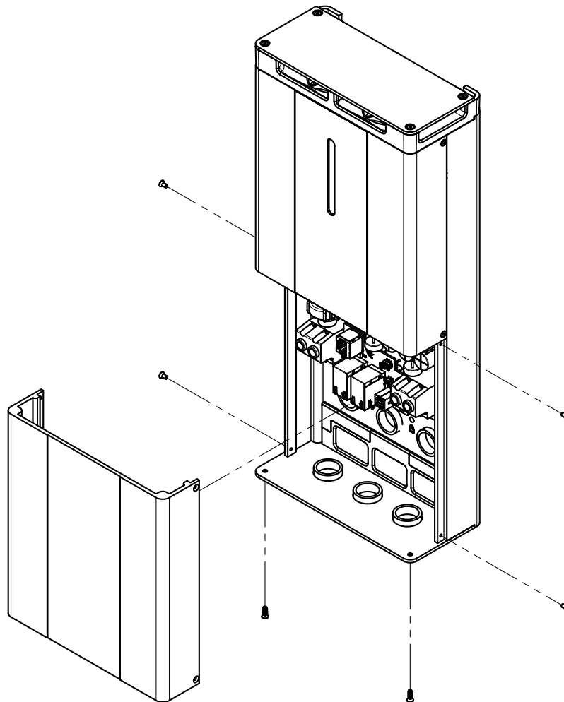
Figure 2: SRX Access Panel Screw Locations
