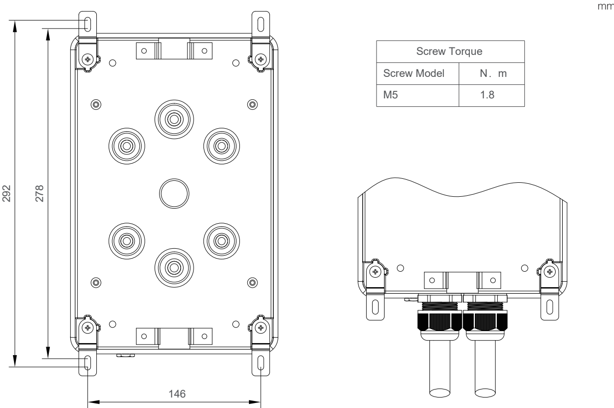
Fig 2 2-in 2-out mounting sizes drawings
