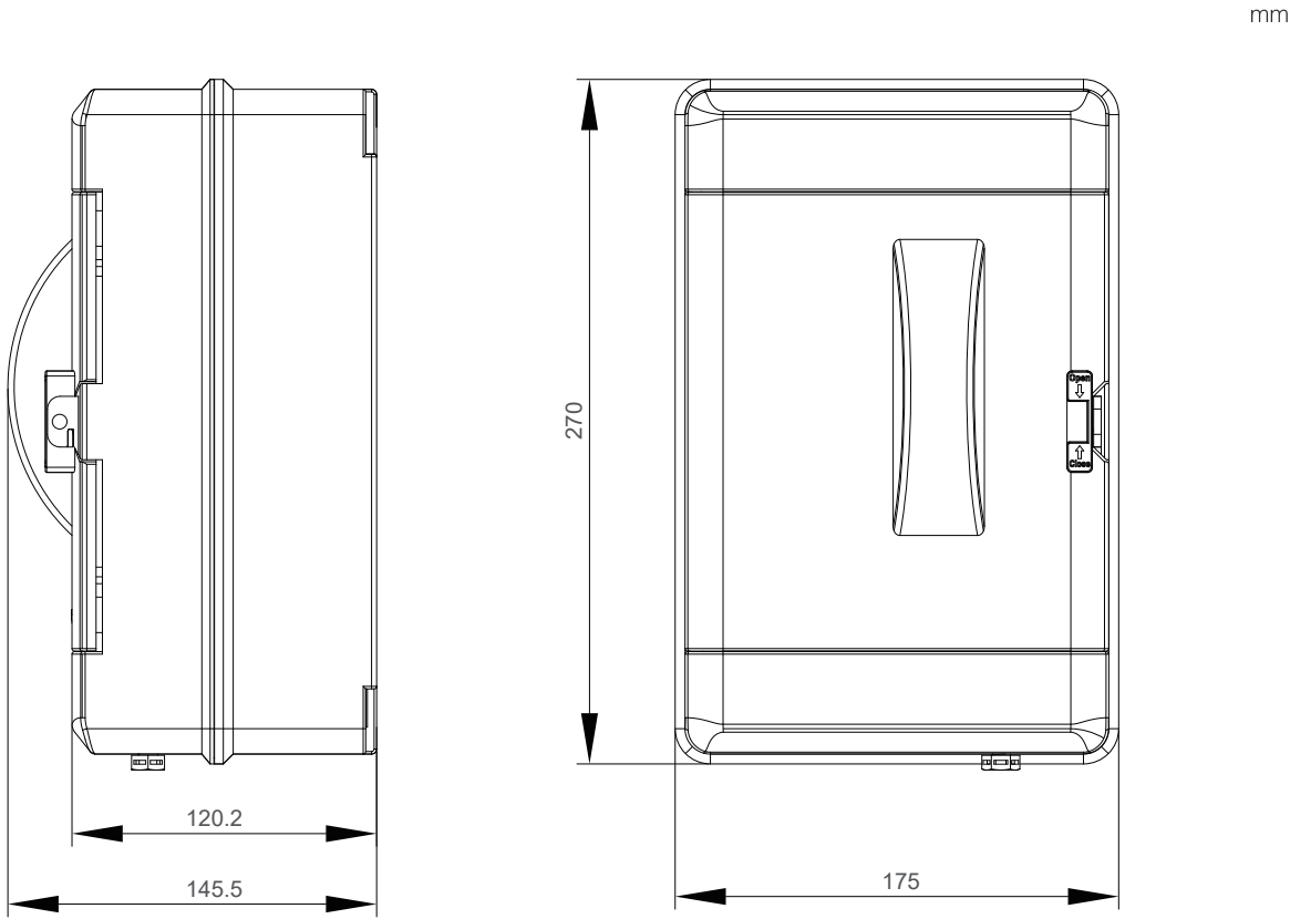
Fig 1 WPB outline sizes drawings
