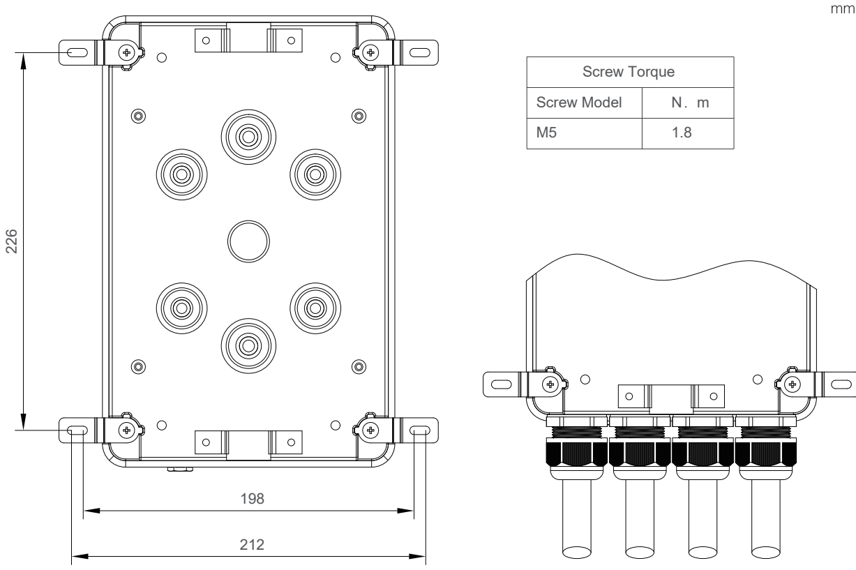
Fig 3 2-in 4-out mounting sizes drawings
